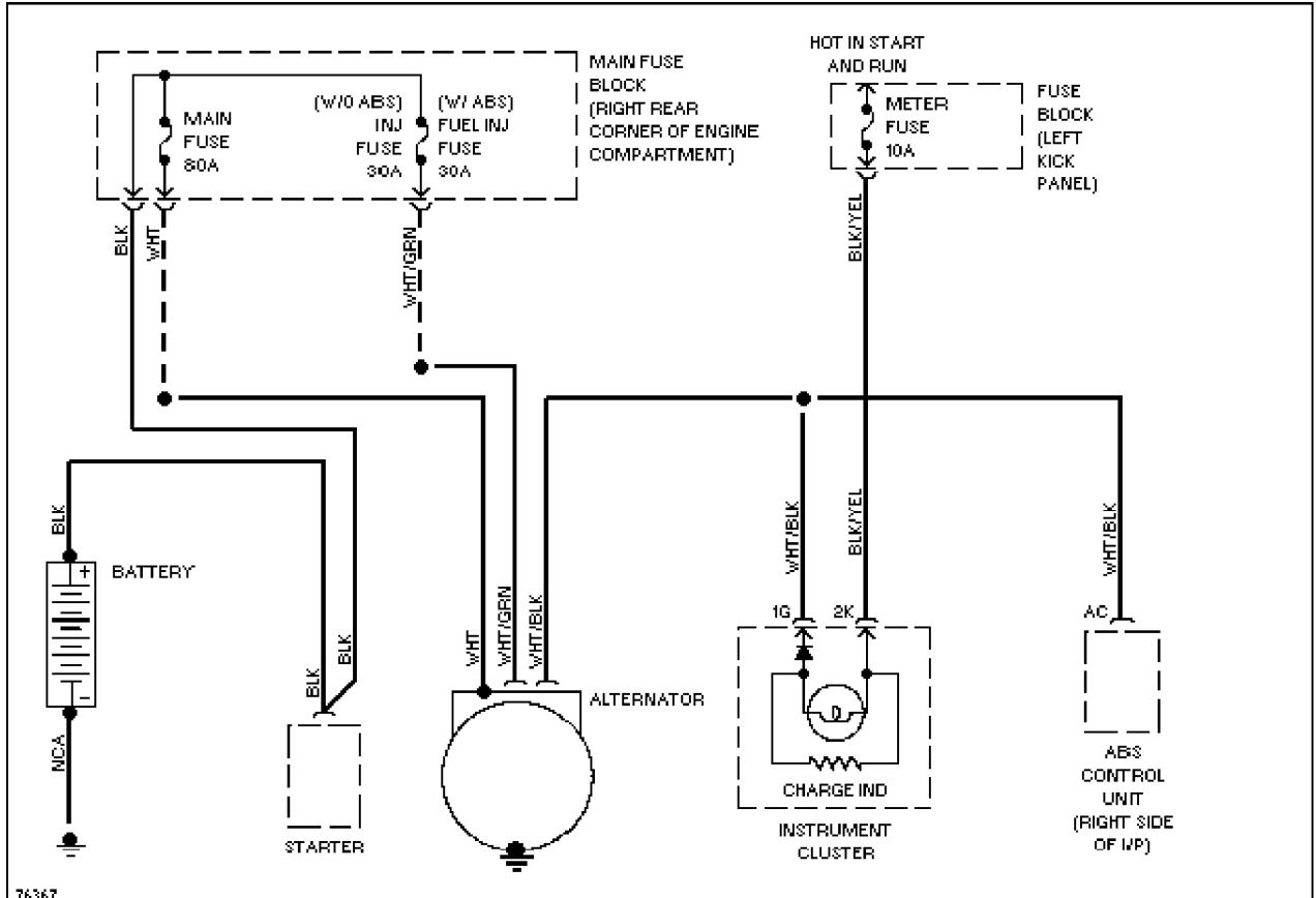
76367 Charging Circuit
