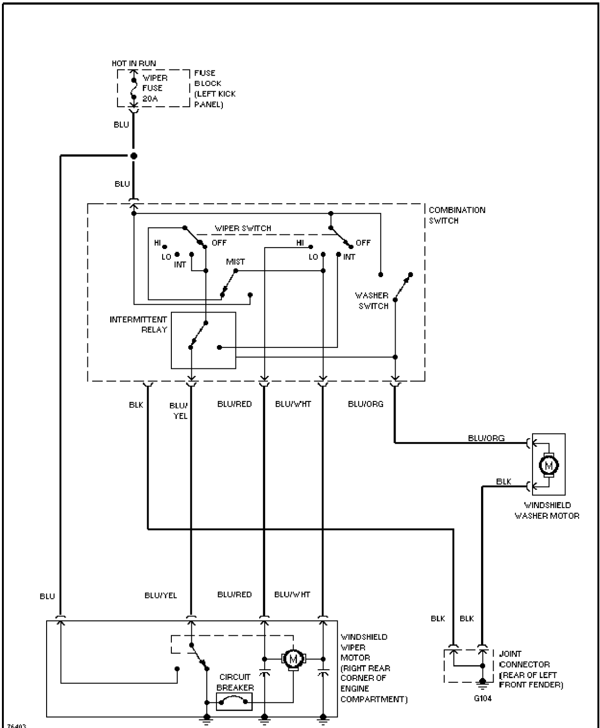
Wiper/Washer Circuit
